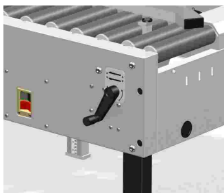
Crank handle adjustment for case size.
