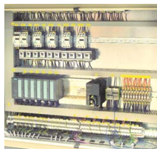
Well organised control cabinets with space for expansion.
